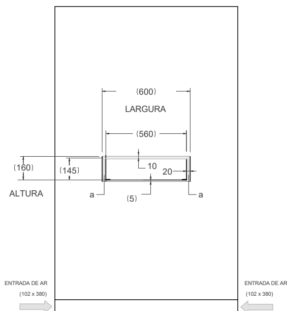
VISTA FRONTAL
